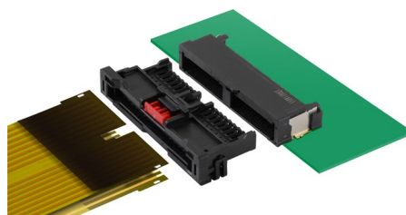
Double-Cable Version
