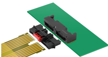
Single-Cable Version
