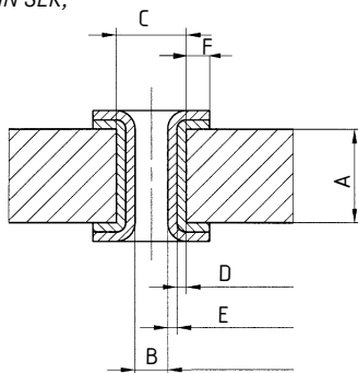
Figure XII-2: Schematic view of the circuit board's hole layout, 6 mm hole
