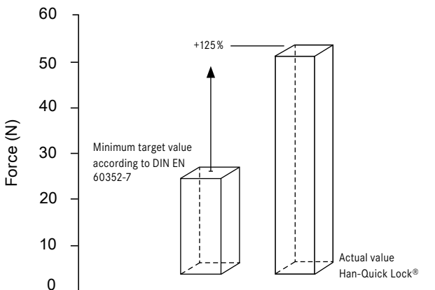
Figure VIII-4: Wire pull-out forces with cable cross-section 0.5 \text{ mm}^2
