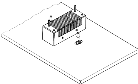
Figure XII-8: Holding block configured to hold connectors
