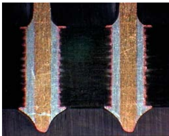
Figure IX-7: Plated through-hole with connector termination
