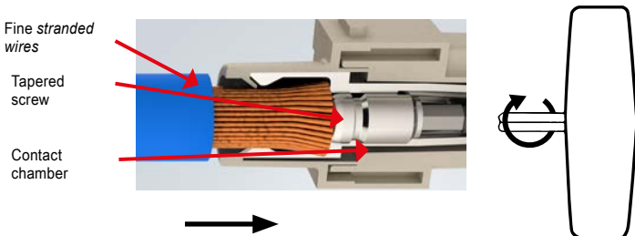
Figure III-3: Schematic view of a standard axial screw contact
