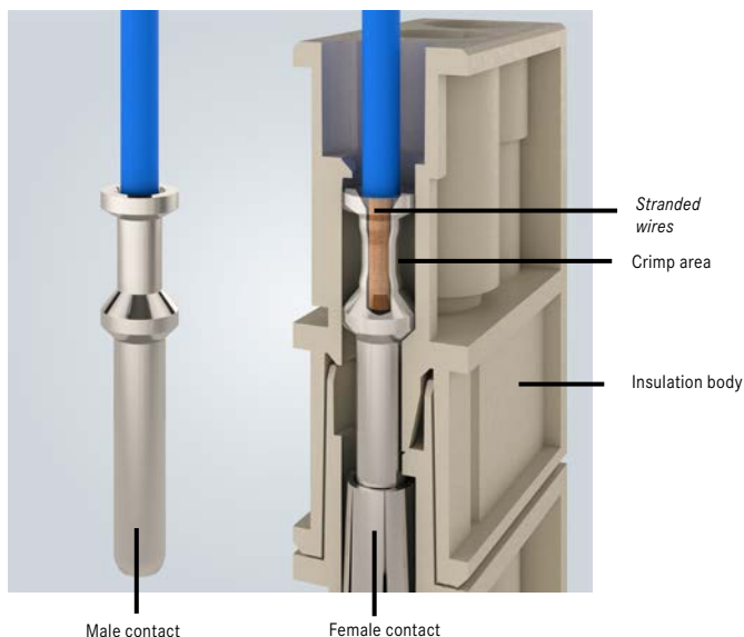
Termination principle of crimp technology
