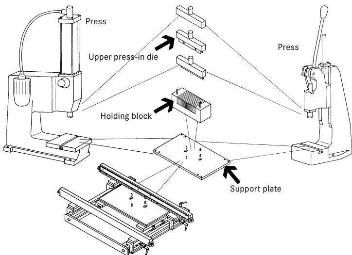
Figure XII-6: Construction of HARTING's modular tool system
