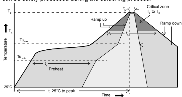
Figure IX-2: Soldering profile measured on the component, acc. to IPC-Jedec J-Std 020C
