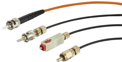
Figure VII-5: F-SMA and F-ST connectors, SC contact (2 nd f.r.)
