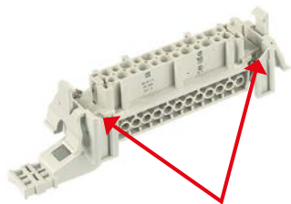
Figure II-10: Insert with Han-Snap®: The PE panels are not electrically connected to each other (refer to red arrows)
