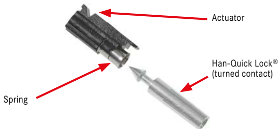
Figure VIII-1: Actuator and radial clamp of the Han-Quick Lock®
