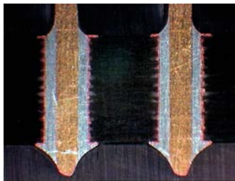
Figure IX-9: Properly soldered joint
