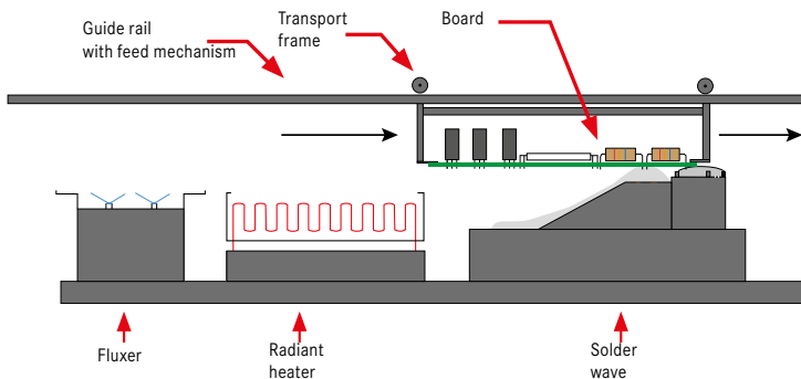
Figure IX-1: Principle of wave soldering
