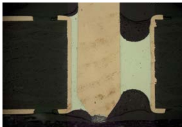
Figure IX-10: Soldered joint with marginal fill level
