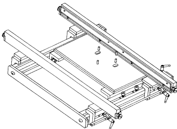
Figure XII-9: Guide frame that positions the circuit board for the press-in die
