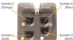
Figure XI-17: Rear view of data module
