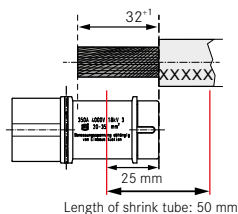
Figure VIII-2: Cage-clamp termination
