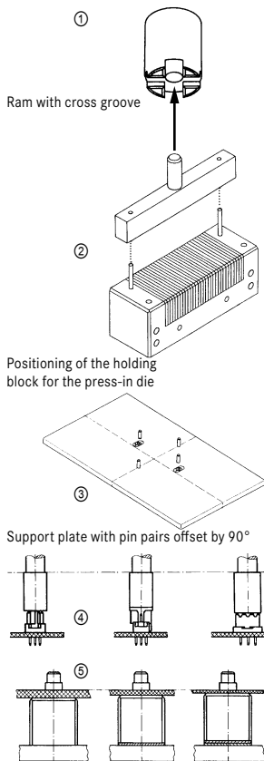
Different contacts pressed into PCBs
