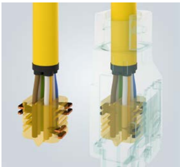
preLink ® termination technique, with transparent terminal module
