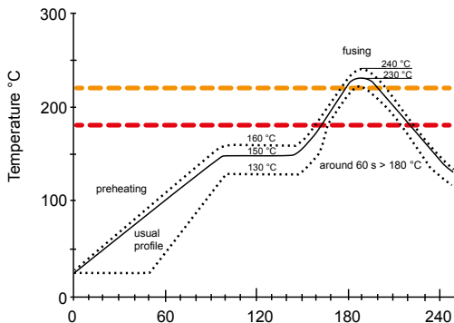
Figure IX-3: Soldering profile for reflow soldering (temperature at the solder joint)
