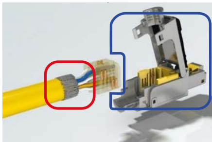
Figure XI-20: preLink® terminal module, RJ 45 mating face
