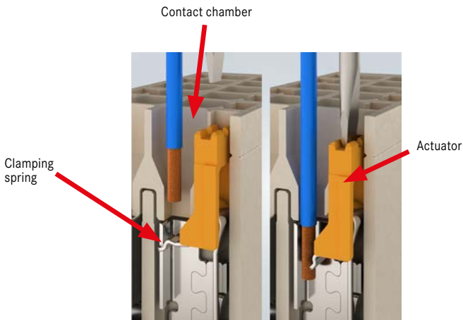
Figure VII-1: Contact chamber Han® Push-In module with termination
