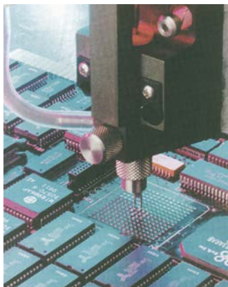
Figure IX-6: Dispenser in use
