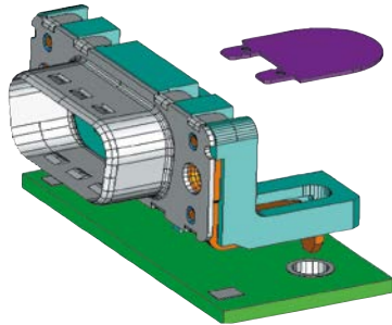
Figure IX-4: D-Sub THR connector
