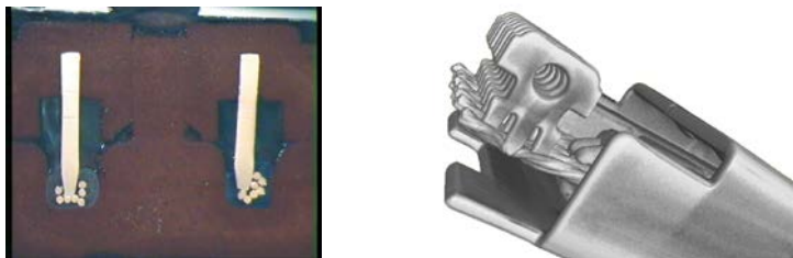
Figure XI-21: Micro-section of piercing termination technique
