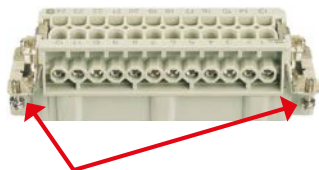
Figure II-8: Unmounted insert: The PE panels are not electrically connected to each other (refer to red arrows)
