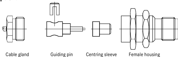
Figure XIII-9: F-TNC female
