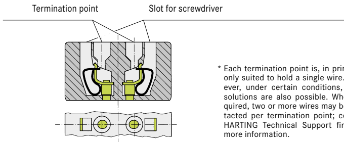
Figure VI-3: Structure of termination point with cage-clamp
