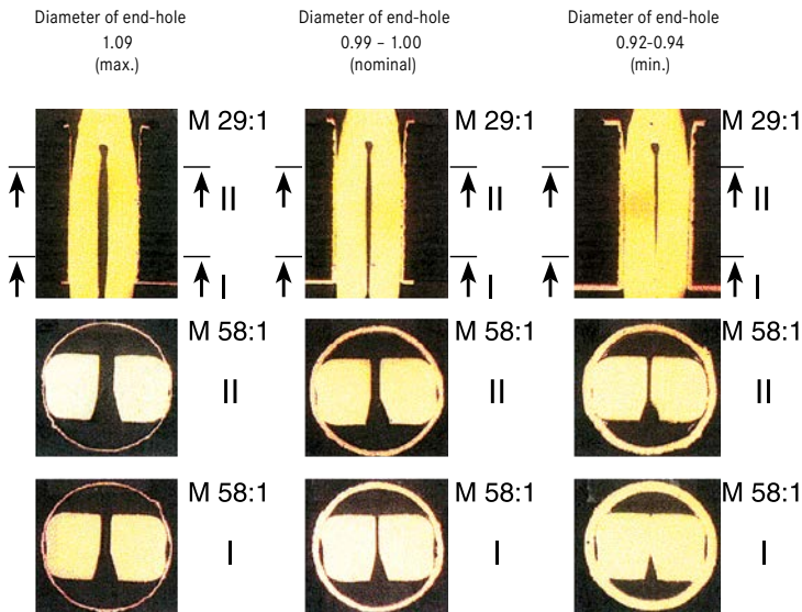
Figure XII-6: Cross-sectional images of a 2.4 mm thick circuit board, varying hole diameters
