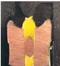
Figure XI-23: Contact with a solid wire core
