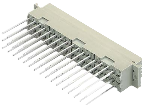
Figure X-1: DIN 41612 type F with wrapping posts
