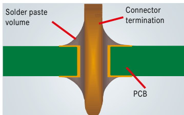
Figure IX-7: Plated through-hole with connector termination
