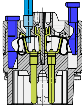
Fig. VI-1: Termination principles of standard cage-clamp Ⓐ and Han ® ES Press Ⓑ
